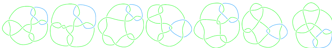
L10a8
