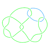
L11a85
