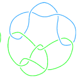
L11a84
