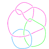
L11n278
