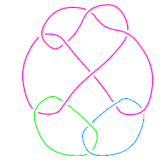
L11n257
