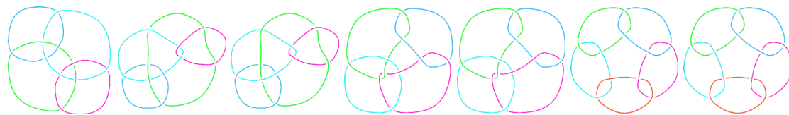
L10n107
