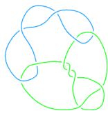
L11a86
