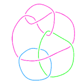
L11n277
