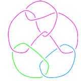
L11n259
