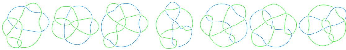
L10n51
