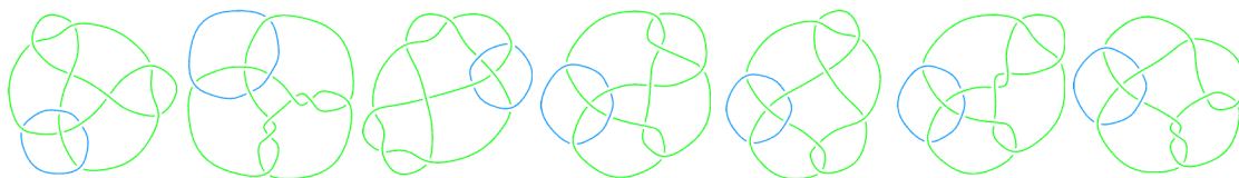
L11a8
