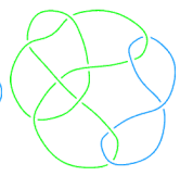
L11a70
