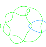
L11a111
