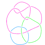
L11n283
