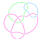
L11n296
