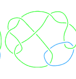
L11a83
