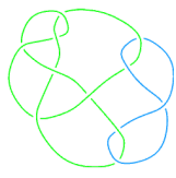
L11a78
