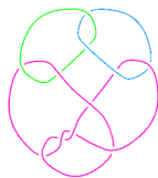
L11n272
