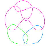
L11n262
