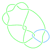
L11a64
