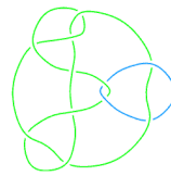
L11a69
