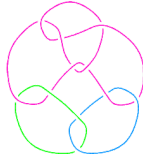
L11n258
