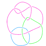
L11n284
