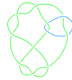
L11a76
