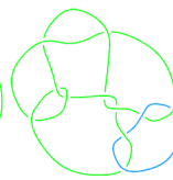
L11a89
