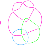
L11n288
