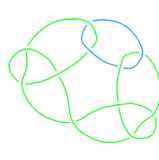
L11a95
