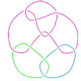
L11n260
