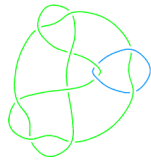
L11a71
