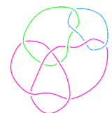
L11n295
