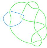
L11a74
