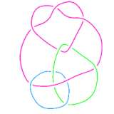
L11n289
