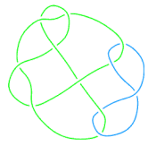
L11a77
