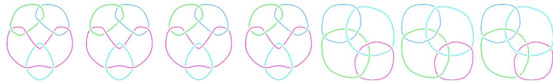
L10n100
