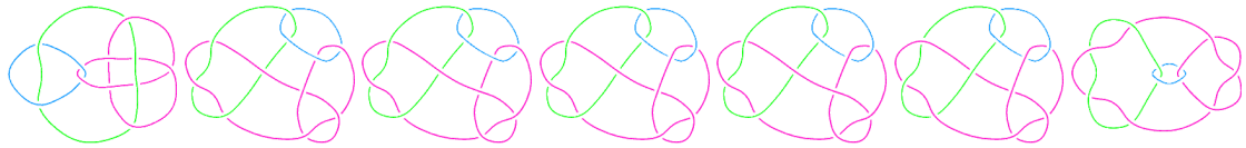
L11n300 L11n301 L11n302 L11n303 L11n304 L11n305 L11n306
