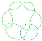
L11a99
