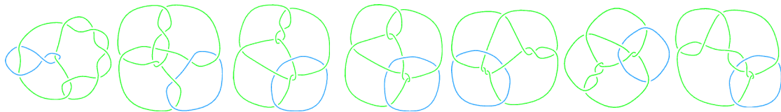
L11a43 L11a44 L11a45 L11a46 L11a47 L11a48 L11a49
