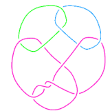
L11n273
