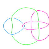
L11n298
