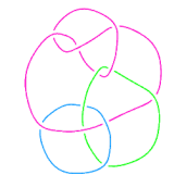
L11n276
