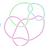
L11n294
