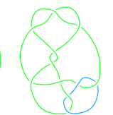
L11a109
