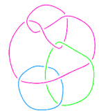
L11n279
