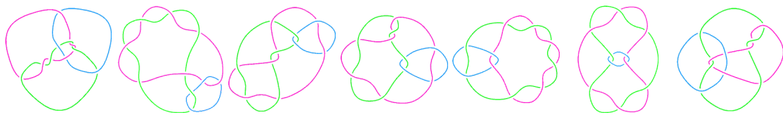
L10a141 L10a142 L10a143 L10a144 L10a145 L10a146 L10a147
