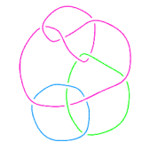
L11n281
