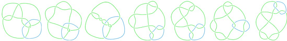
L10a22
