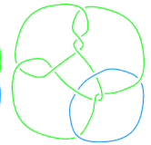
L11a98
