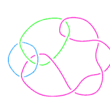
L11n285
