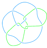
L11n251
