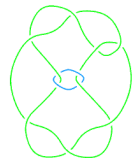
L11a68
