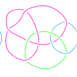
L11n292
