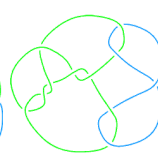
L11a90
