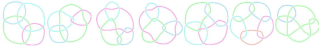
L10a169 L10a170 L10a171 L10a172 L10a173 L10a174 L10n1
