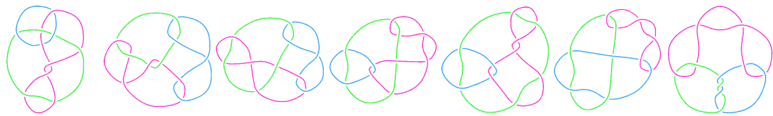
L10a127 L10a128 L10a129 L10a130 L10a131 L10a132 L10a133
