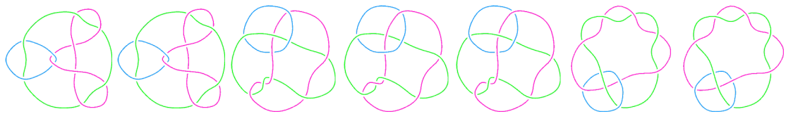
L10n72
