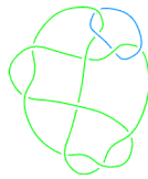
L11a65
