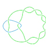
L11a110
