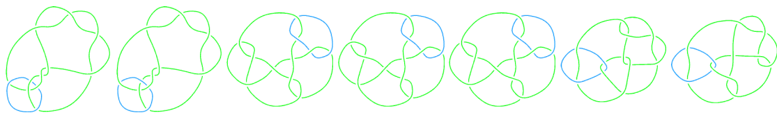
L11n48
