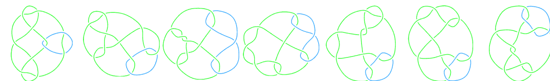
L11a57 L11a58 L11a59 L11a60 L11a61 L11a62 L11a63
