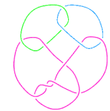
L11n271
