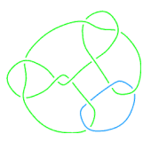
L11a92
