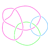
L11n293
