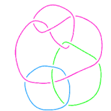
L11n280
