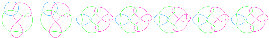
L11n335 L11n336 L11n337 L11n338 L11n339 L11n340 L11n341
