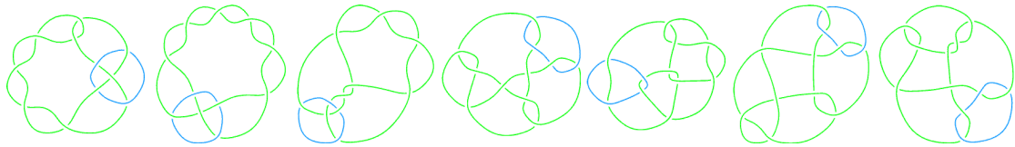
L11a15 L11a16 L11a17 L11a18 L11a19 L11a20 L11a21
