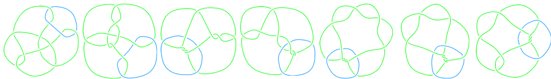
L11n76
