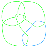
L11a80
