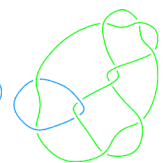
L11a112
