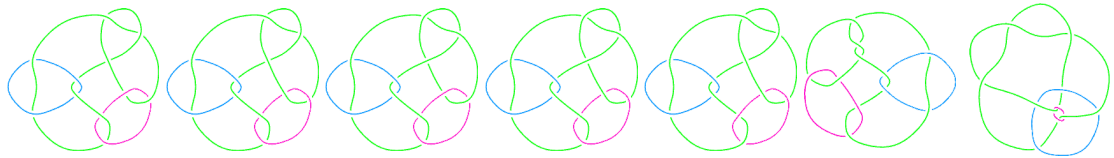
L11n398 L11n399 L11n400 L11n401 L11n402 L11n403 L11n404
