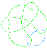
L11a79
