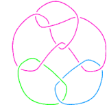
L11n263
