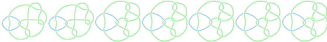
L11n55
