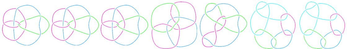
L11n433 L11n434 L11n435 L11n436 L11n437 L11n438 L11n439
