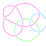
L11n291
