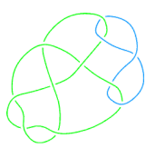
L11a106
