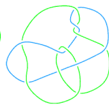
L11n252
