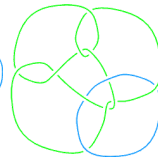
L11a97
