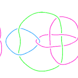
L11n299
