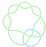
L11a100
