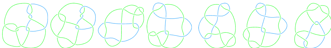
L10a57
