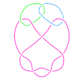
L11n268
