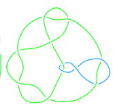
L11a105
