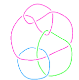
L11n274
