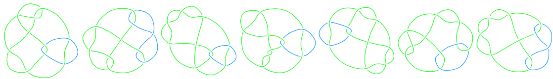
L10a29
