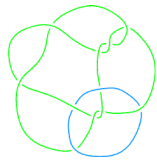
L11a101
