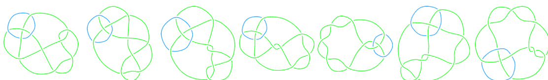
L11a1
