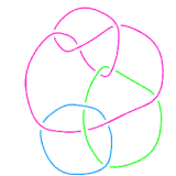
L11n282
