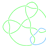
L11a82
