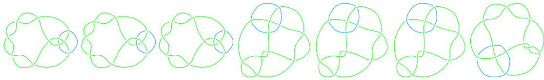
L11n13
