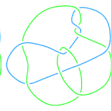
L11n253
