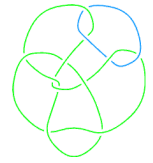
L11a81
