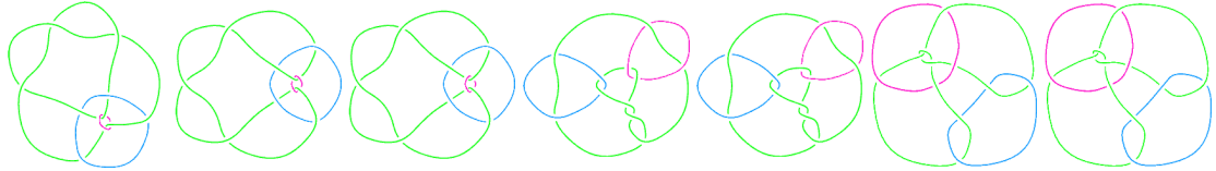
L11n405 L11n406 L11n407 L11n408 L11n409 L11n410 L11n411
