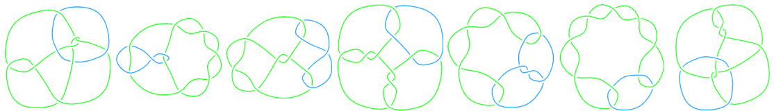
L10a43
