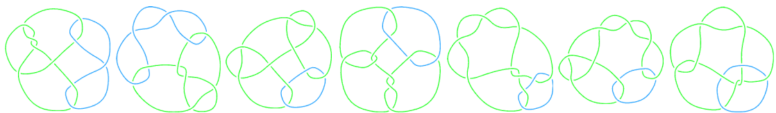
L10a36
