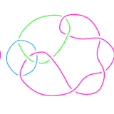
L11n287
