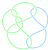
L11a87
