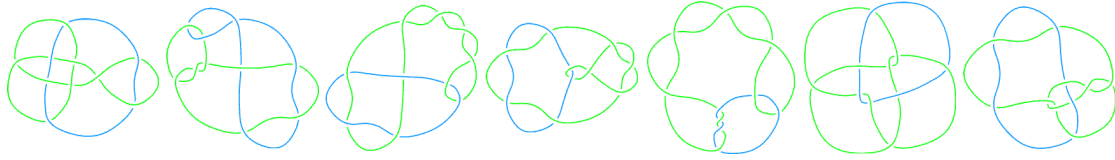
L10a71 L10a72 L10a73 L10a74 L10a75 L10a76 L10a77
