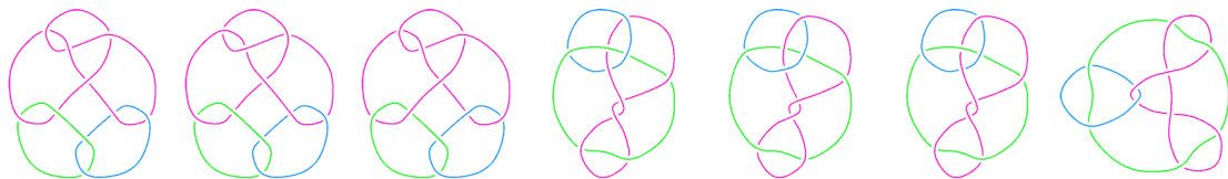
L10n65
