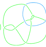
L11a104
