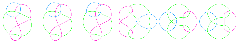
L9n23
