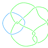
L11a102
