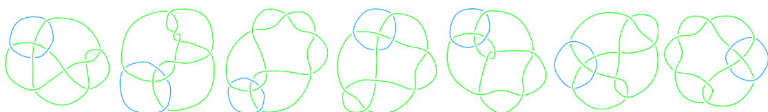
L10a1
