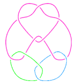
L11n265
