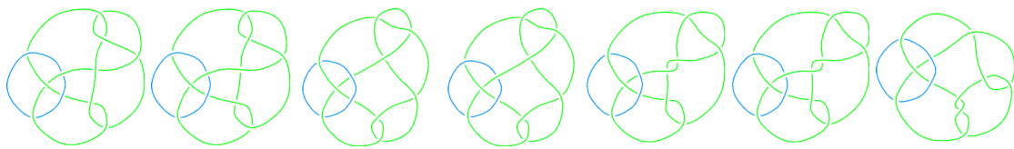
L11n34
