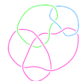
L11n297
