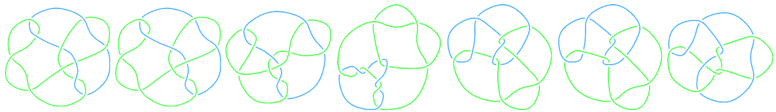
L11n230 L11n231 L11n232 L11n233 L11n234 L11n235 L11n236
