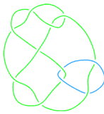
L11a66
