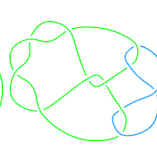
L11a96
