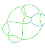
L11a73
