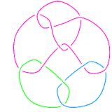
L11n264
