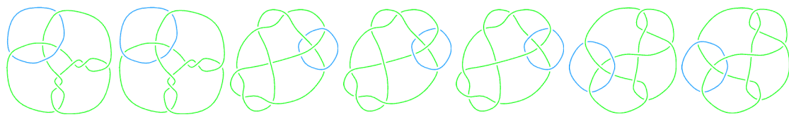
L11n27
