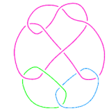
L11n255
