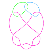
L11n269
