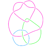
L11n290
