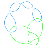
L11a94
