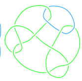
L11a91
