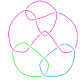
L11n261
