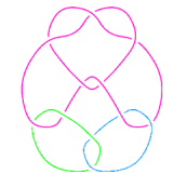
L11n266
