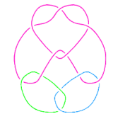
L11n267
