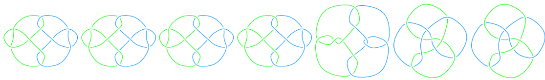
L10n58
