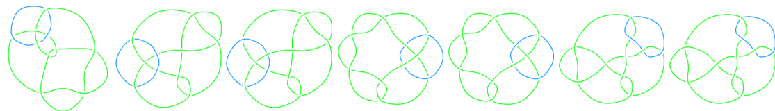
L10n16 L10n17 L10n18 L10n19 L10n20 L10n21 L10n22
