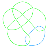
L11a67
