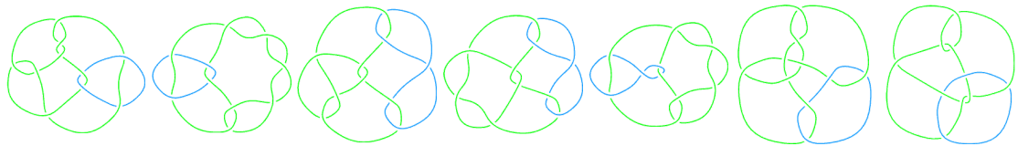
L10a15
