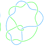
L11n254
