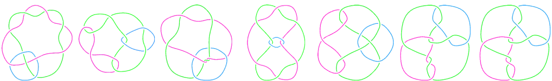
L10n79
