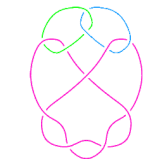
L11n270
