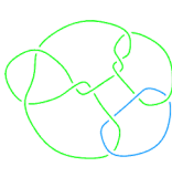
L11a93
