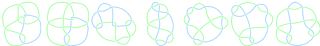
L10a85 L10a86 L10a87 L10a88 L10a89 L10a90 L10a91
