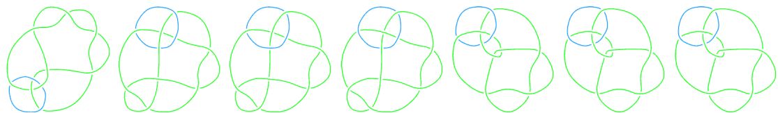
L10n9 L10n10 L10n11 L10n12 L10n13 L10n14 L10n15
