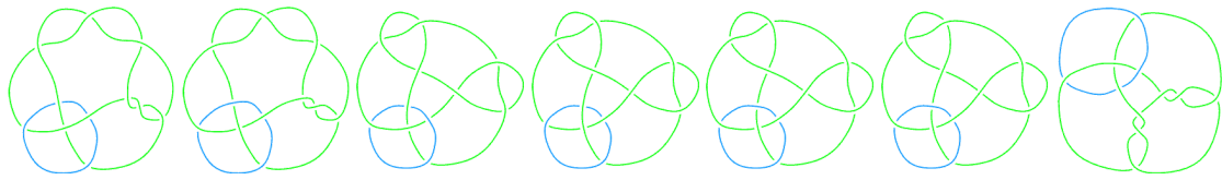
L11n20
