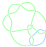
L11a88
