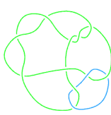
L11a108
