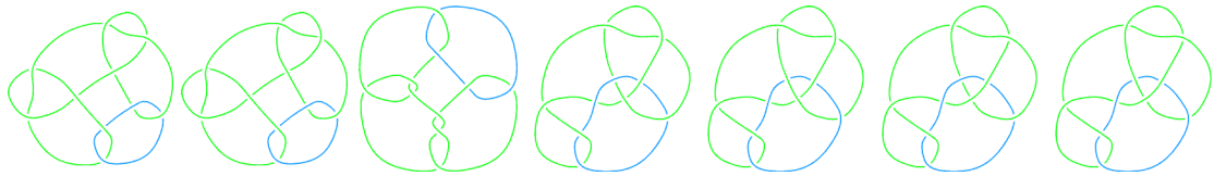
L10n37
