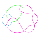
L11n286
