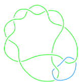
L11a107
