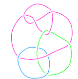
L11n275
