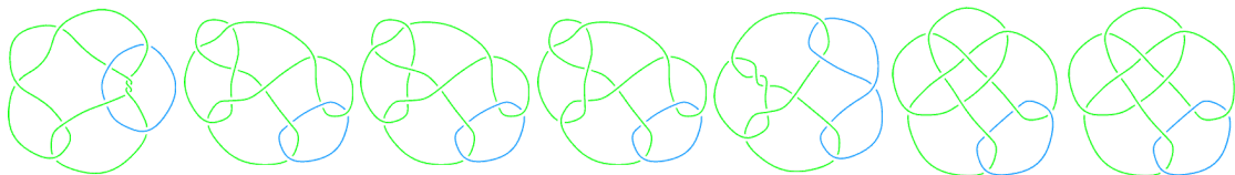
L11n83
