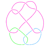
L11n256
