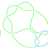
L11a75
