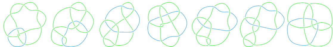
L10a50
